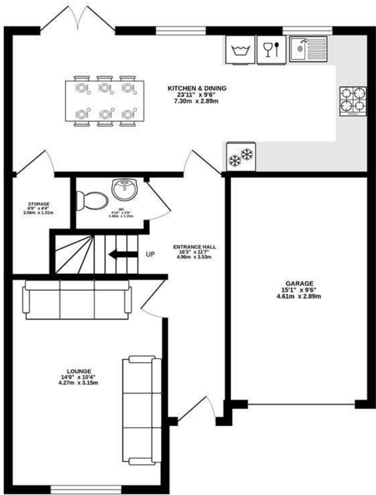
GROUND FLOOR 652 sq.ft. (60.6 sq.m.) approx.
